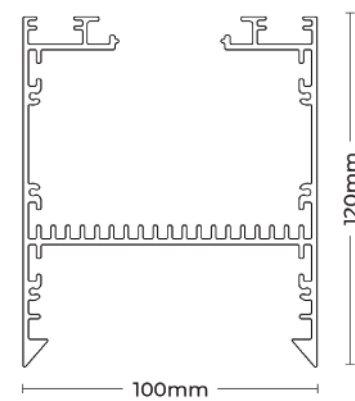
PRODUCT DRAWING
